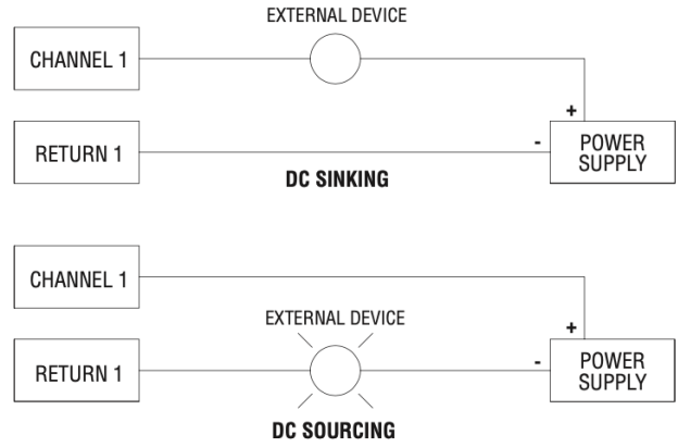
2591-A Typical External Wiring Application
