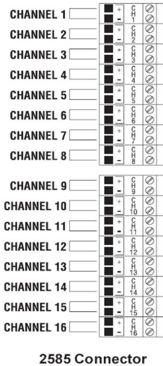
Figure 3 2585 Wiring Connector Diagram
